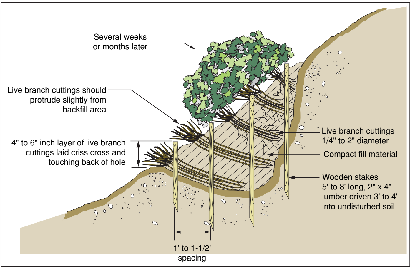
Figure 17—Typical branchpacking. (Lewis 2000)
