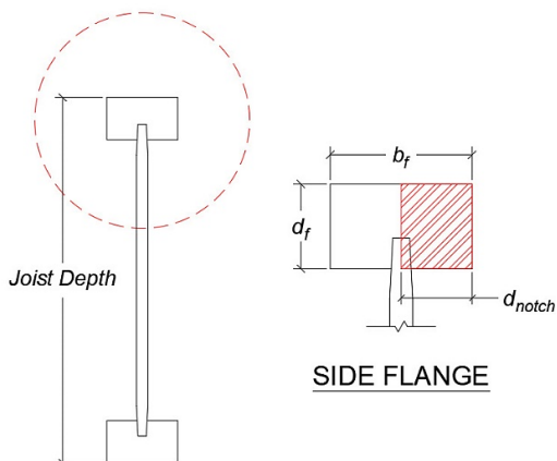
Figure 1: Diagram of an inadvertent Side Flange Notch in top (compression) flange of a TJI® joist.
