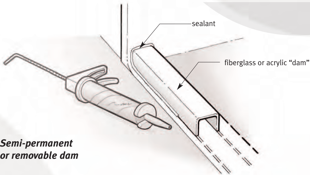
Flexible dams or water retainers
